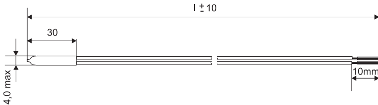
shrink tube housing for monitoring windings
