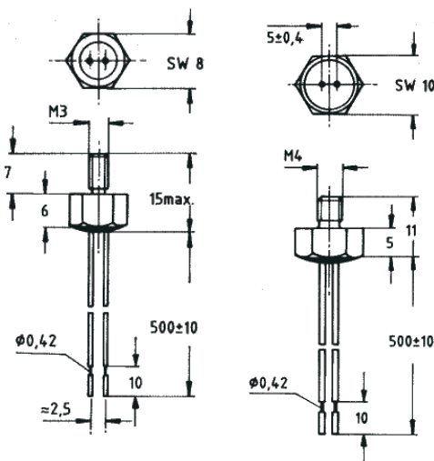
Screw-in sensors in alu-housing SW8-M3 SW10-M4
