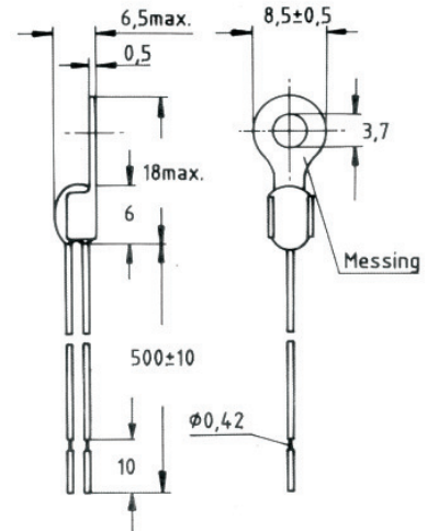
Pt-sensor in cable shoe - surface sensor
