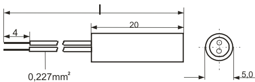
Pt-sensor in stainless steel
