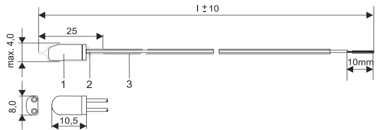
Pt-sensor in cable shoe - surface sensor
