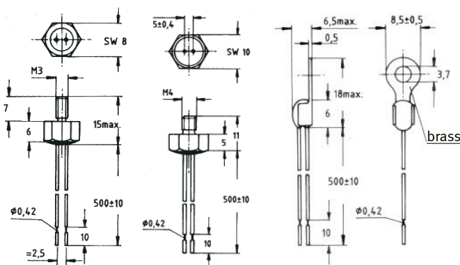
Pt100-screw-in-sensor and surface sensor
