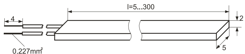
HGW-slot sensor
